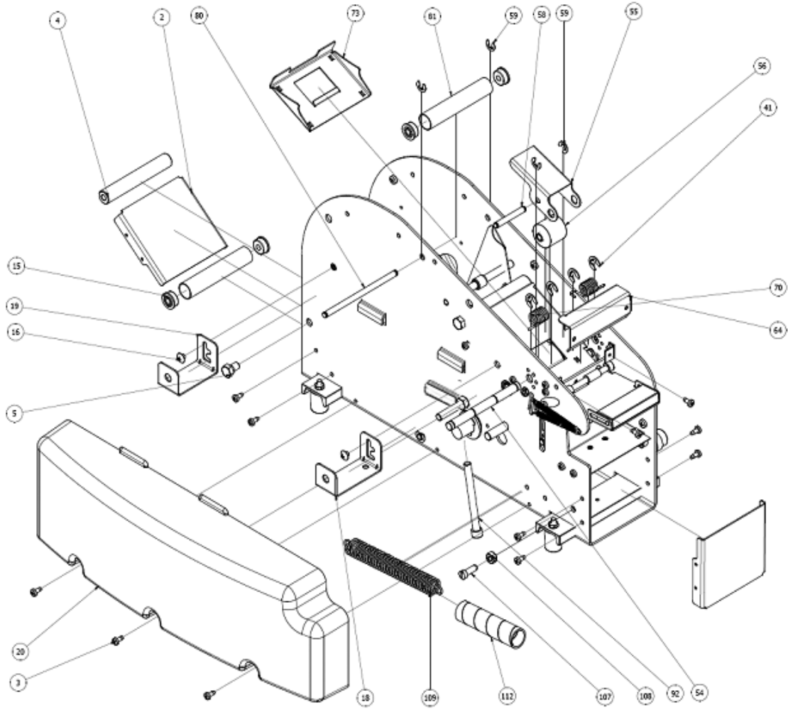
TD2100 Manual Drawing #2
